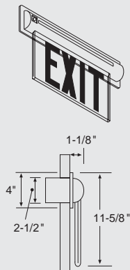
RECESSED WALL MOUNT
