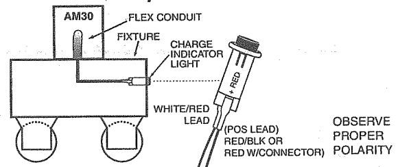
Illustration 2 Strip Fixture
