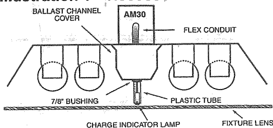
Illustration 1 Recessed Troffer Fixture
